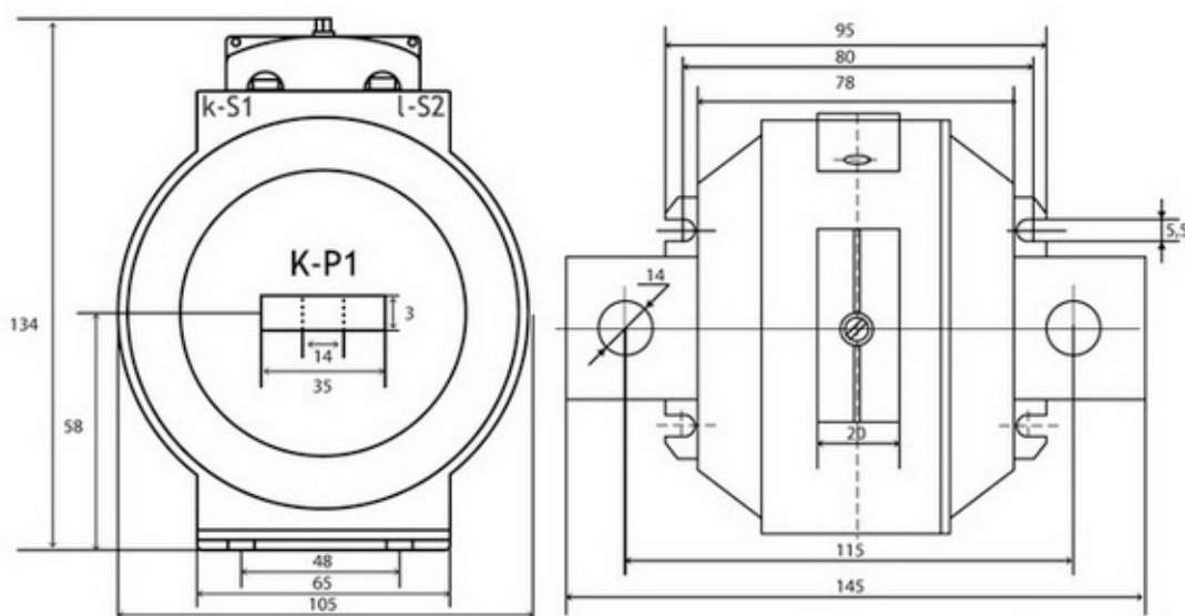
AMT-0-V 5/5-300/5
